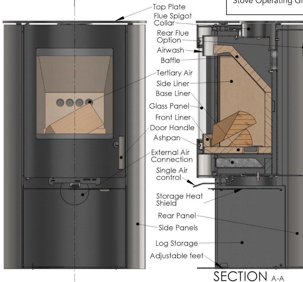
Figure 2 – FCS Stove controls.
