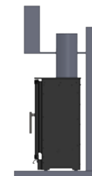
Fig.1 Rigid metal Pipe with Closure Plate
