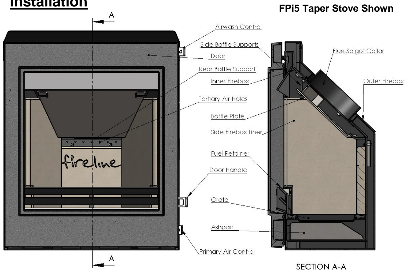
Fig 2 – FGi/FXi/FPi 5 Taper Stove Assembly and controls
